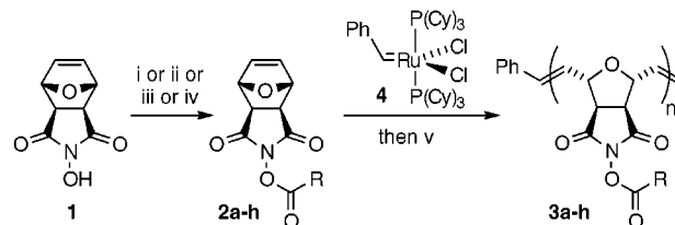
Scheme 1. Synthesis of ROMPGEL Activated Esters
